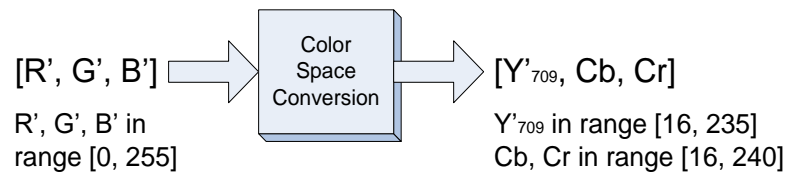
Figure 8-5 : Full scale RGB for BT.709
