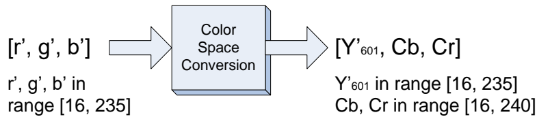
Figure 8-4 : Scaled down rgb for BT.601
