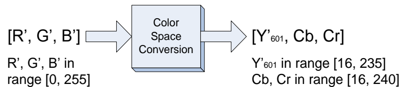
Figure 8-3 : Full scale RGB for BT.601
