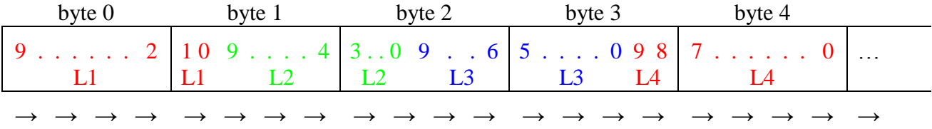
Figure 6-11 : 10-bit monochrome pixel msb packed (Mono10pmsb)
