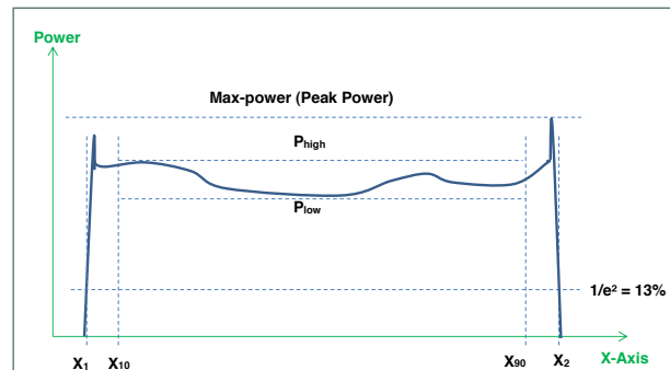
Power Distribution
