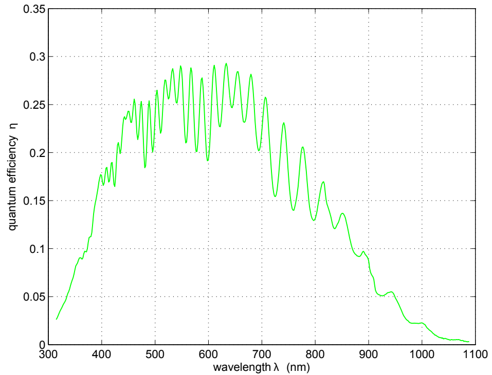
Figure 13: Example for a spectroscopic measurement of the quantum efficiency in a range from 300–1100 nm with a FWHM of 10 nm, no smoothing is applied.
