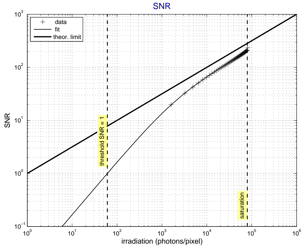
Figure 7: Example of a SNR graph. It contains the measured SNR values, the theoretical curve according to the linear camera model Eq. (11) determined with the measured \sigma_d^2 and \eta values, the theoretical curve according to Eq. (45) including in addition the effect of spatial nonuniformities (DSNU and PRNU), and the SNR curve for an ideal sensor Eq. (13) with no dark and quantization noise and a quantum efficiency \eta of 1. The absolute sensitivity threshold and the saturation capacity are marked by vertical dashed lines.
