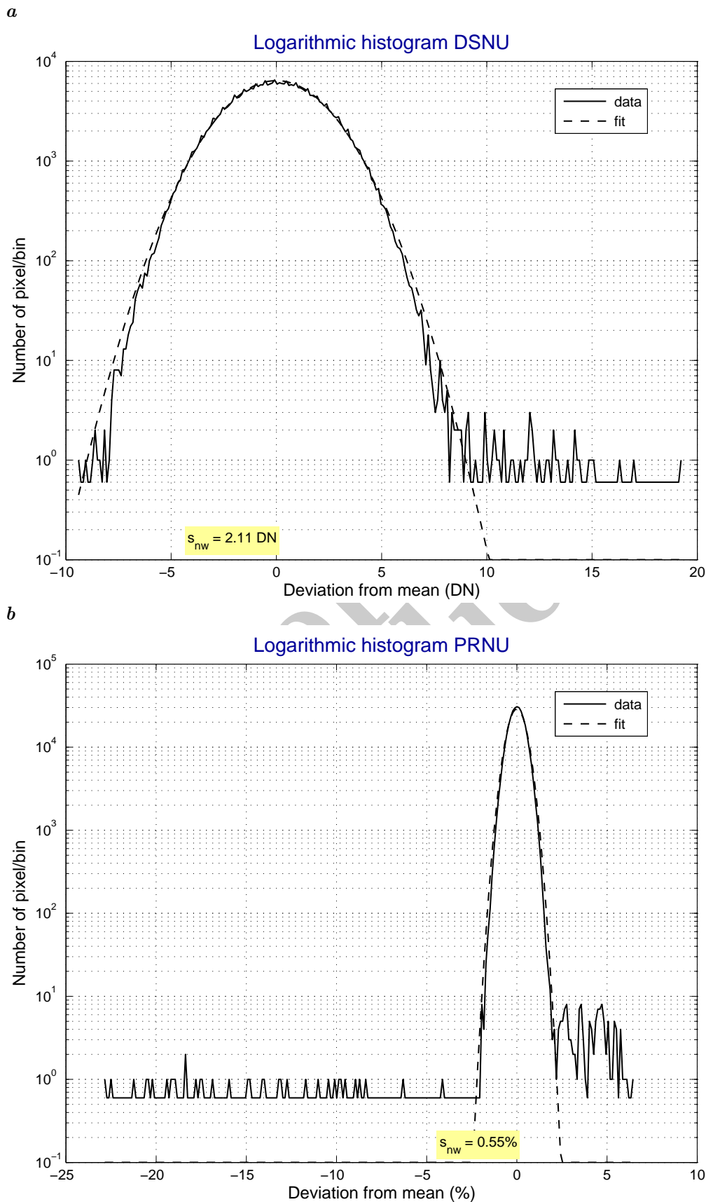
Figure 11: Example for logarithmic histograms for a dark signal nonuniformity (DSNU), b photoresponse nonuniformity (PRNU). The dashed line is the model normal probability density distribution with the non-white standard deviation s_{nw} according to Eq. (50).
